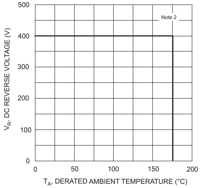
Fig. 6 Operating Temperature Derating
