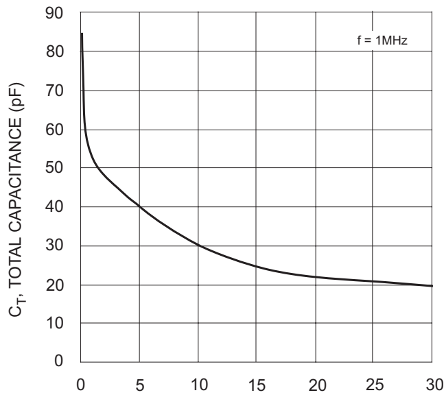
V_R , REVERSE VOLTAGE (V) Fig. 3 Typical Total Capacitance vs. Reverse Voltage
