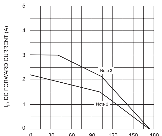
T_A , AMBIENT TEMPERATURE ( ^\circ\text{C} ) Fig. 4 DC Forward Current Derating
